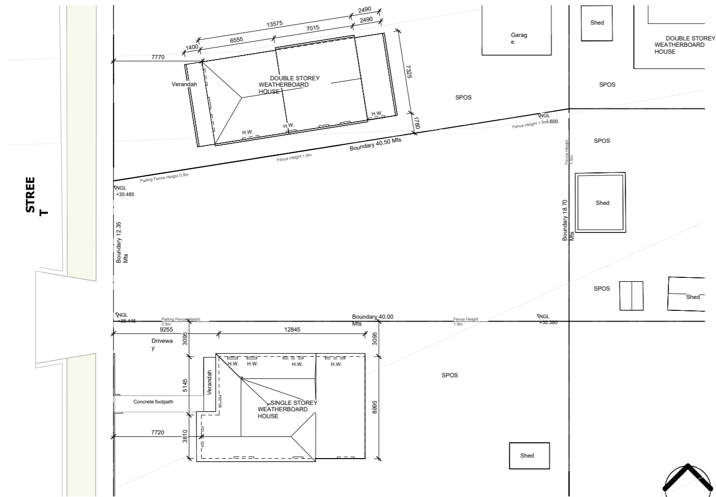
Existing Site Plan scale: 1_100
